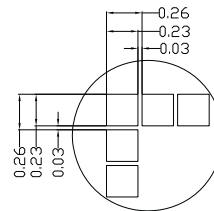
DETAIL A SCALE 20X
